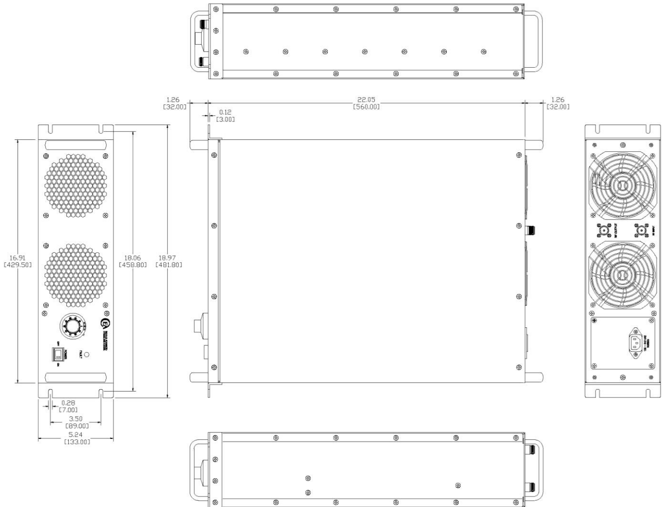
OUTLINE DRAWING - Shown with FGA
