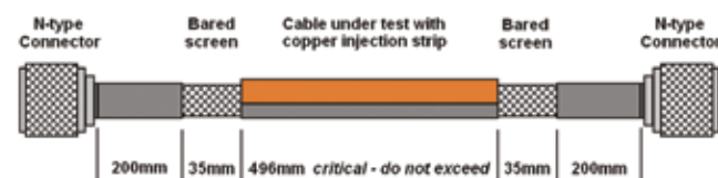
Figure 3. Prepared test sample with injection strip
