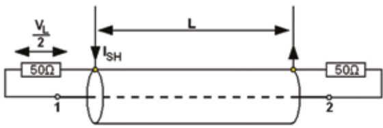
Figure 1. Theoretical arrangement for measuring Z T
