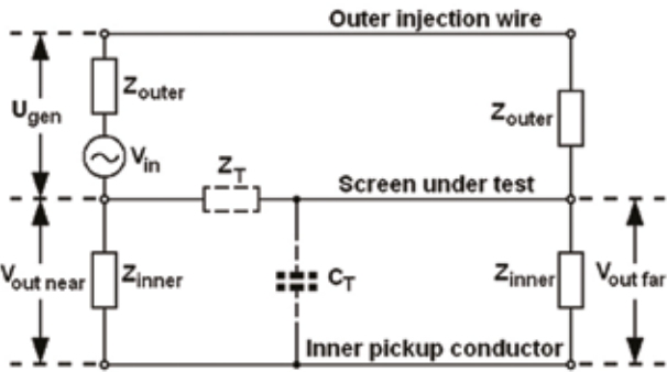
Figure 2. Schematic diagram of line injection method
