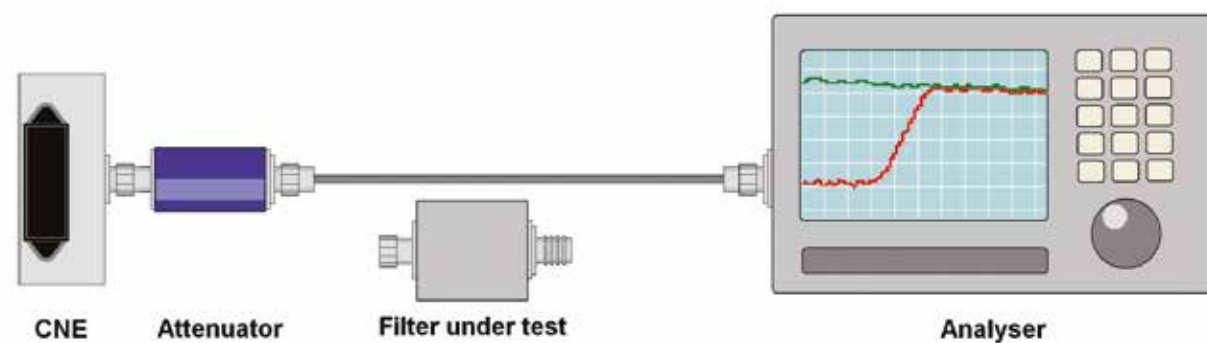
Figure 2. Filter test by substitution setup
