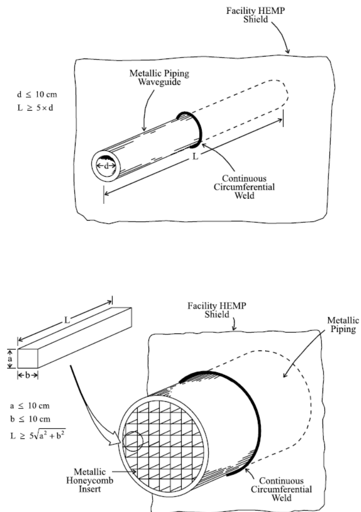
Figure 32. Typical waveguide-below-cutoff (WBC) piping POE protective design for E1 HEMP
