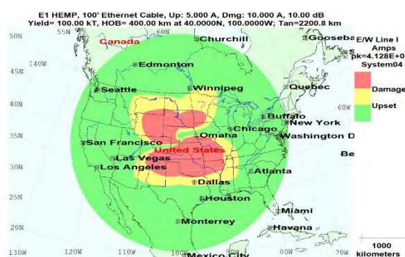
Figure 42. Reduced damage with 10 dB protection to 100' Ethernet cable connected equipment
