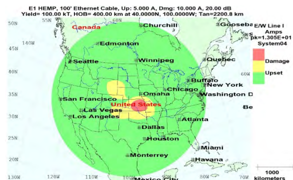
Figure 43. Localized damage only with 20 dB protection with 100' Ethernet cable
