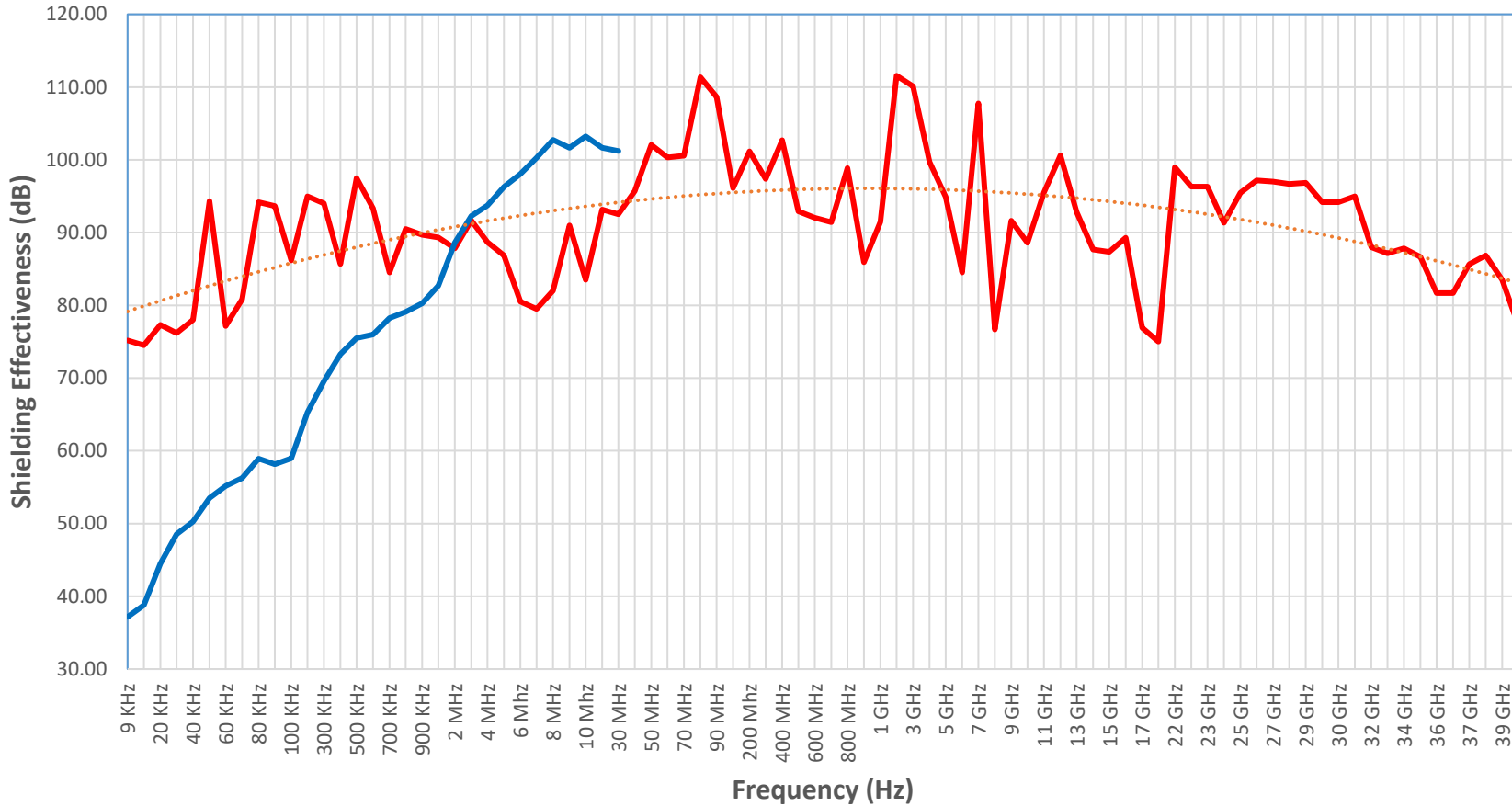
CU50 Shielding Effectiveness (Butt Joint Seam Taped) Tested per IEEE-299 : 2006
