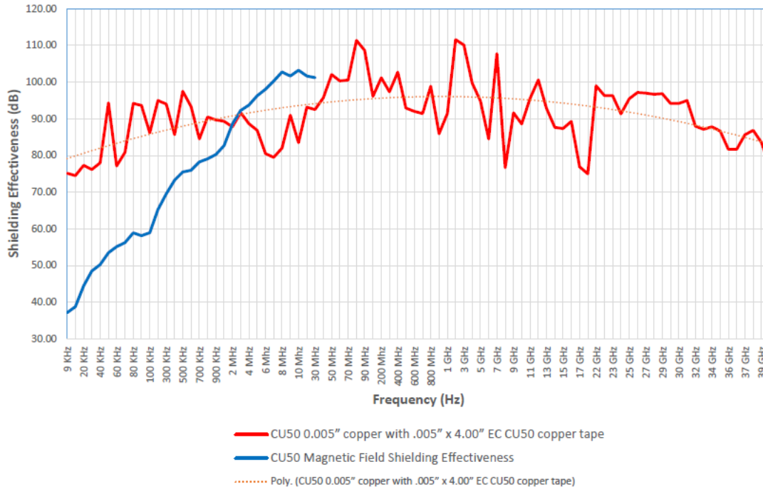
CU50 Shielding Effectiveness (Butt Joint Seam Taped) Tested per IEEE-299 : 2006
