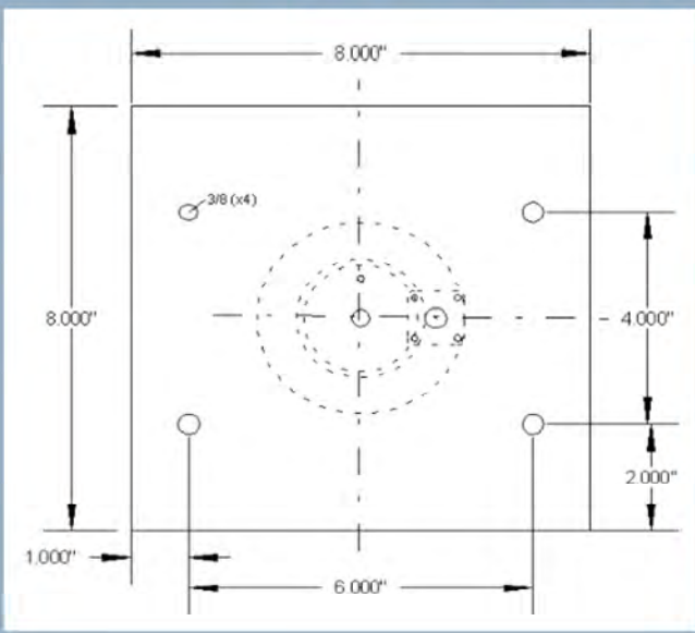
Mounting Dimensions
