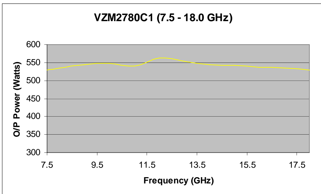
Figure 4(c): VZM2780C1 (8.0-18.0GHz, 500-Watts) O/P Power versus Frequency
