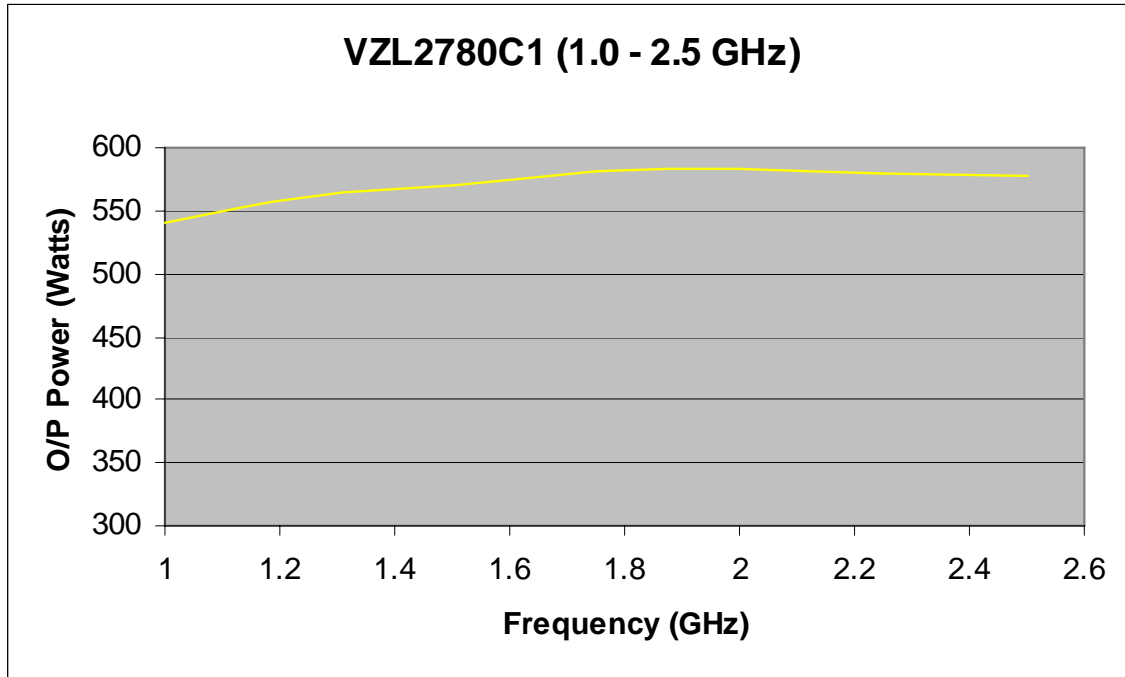
Figure 4(a): VZL2780C1 (1.0-2.5GHz, 500-Watts) O/P Power versus Frequency
