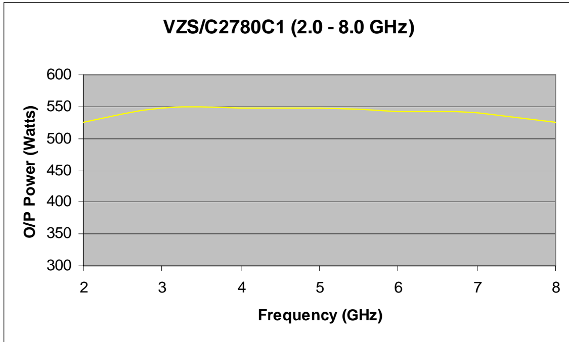
Figure 4(b): VZS/C2780C1 (2.5-7.5GHz, 500-Watts) O/P Power versus Frequency
