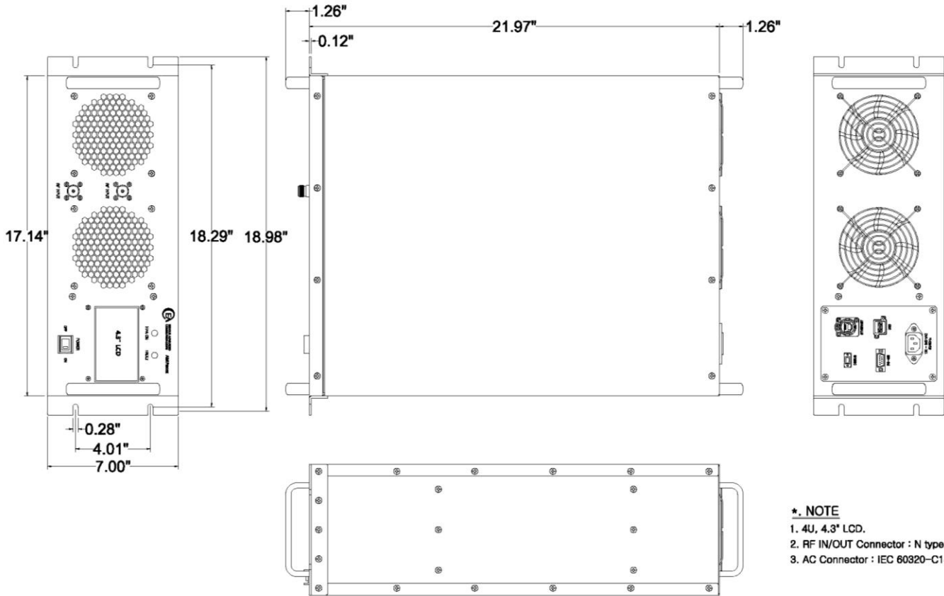
OUTLINE DRAWING SHOWN WITH OPTIONAL LCD CONTROLLER
