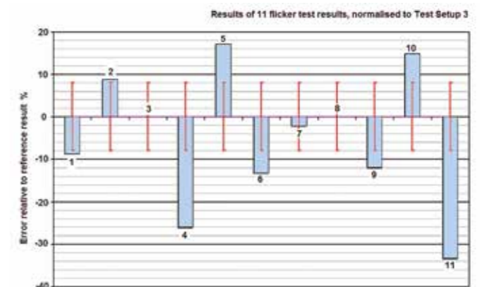
Figure 3. Variance in measurement across flicker tests
