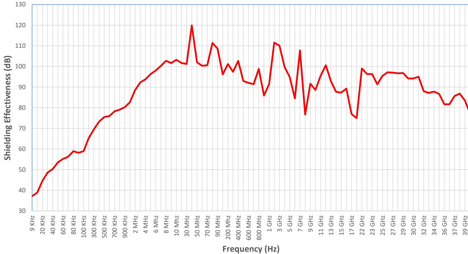
CU50 Shielding Effectiveness (Butt Joint Seam Taped) Tested per IEEE-299 : 2006
