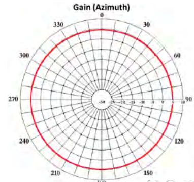
Gain (Azimuth)
