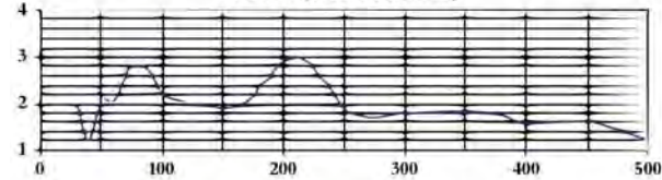
VSWR (0 to 500 MHz)
