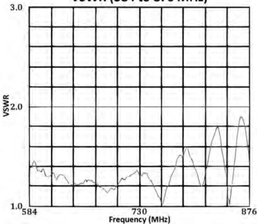
VSWR (584 to 876 MHz)
