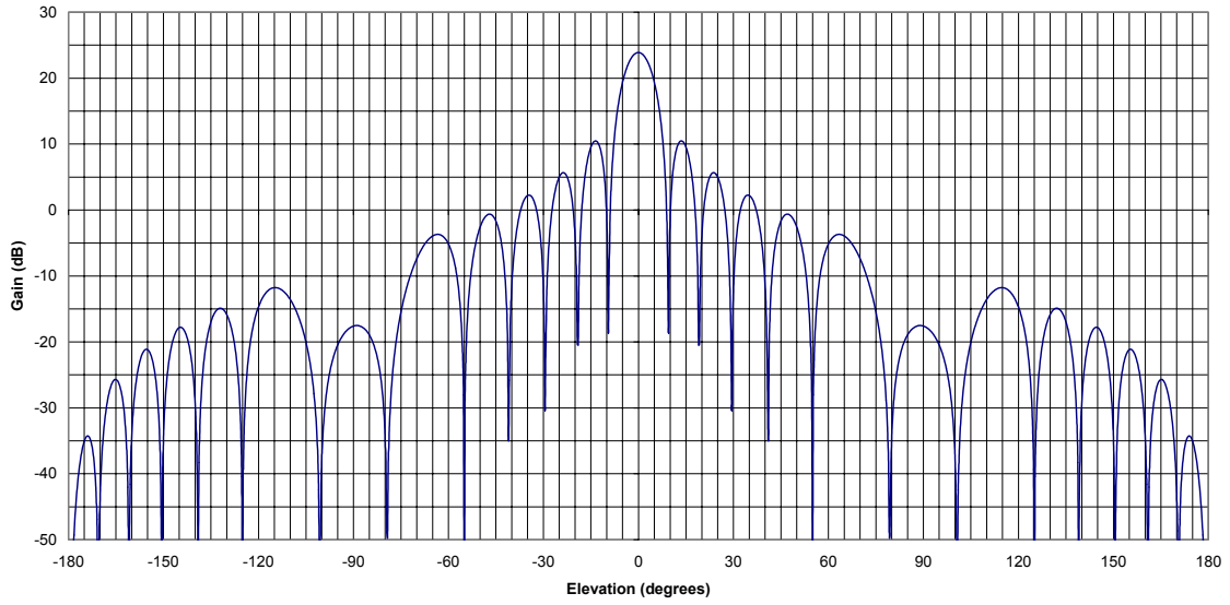
TMC Design Corporation HO-90-24 (10.3 GHz)
