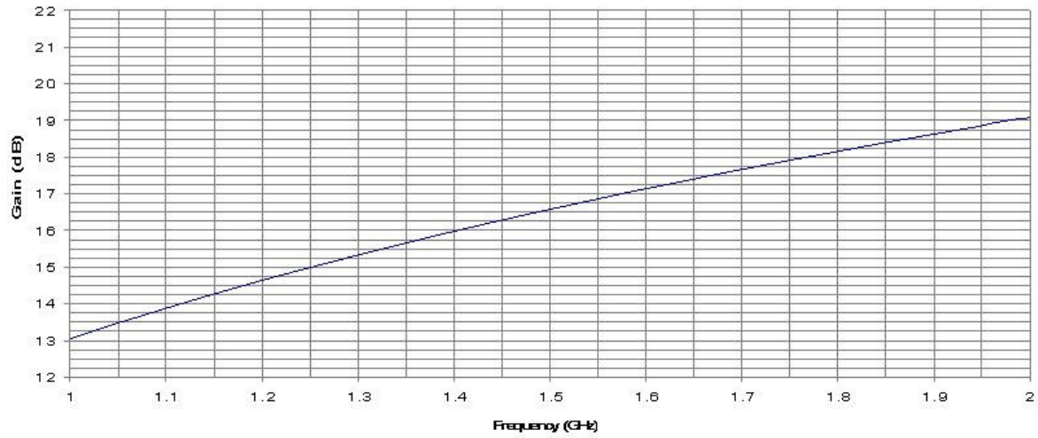
24" Dish with BF-550 (1.5 GHz)
