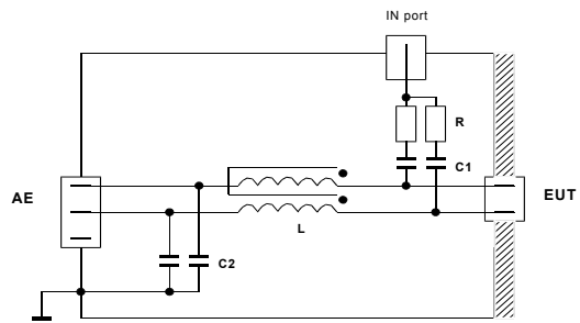
Typical circuit diagram shown with two lines
