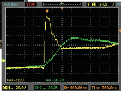
Typical modification of edge of the drive pulse
