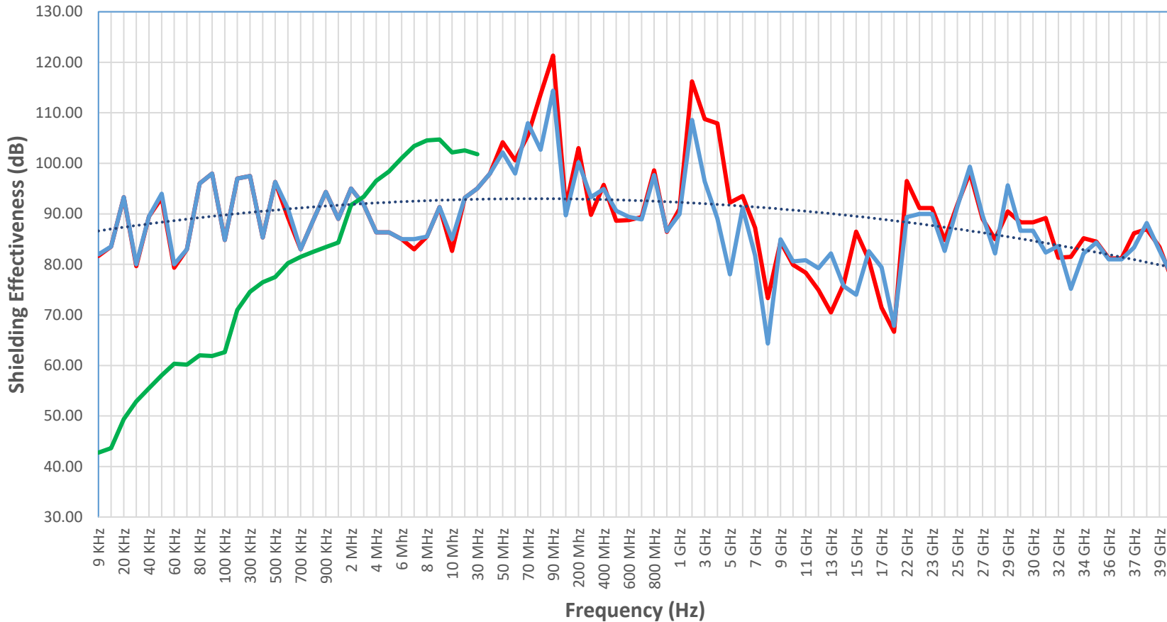
Xalon X250 Panels RF Shielding Effectiveness (Butt Joint & Taped) Tested per IEEE-299 : 2006
