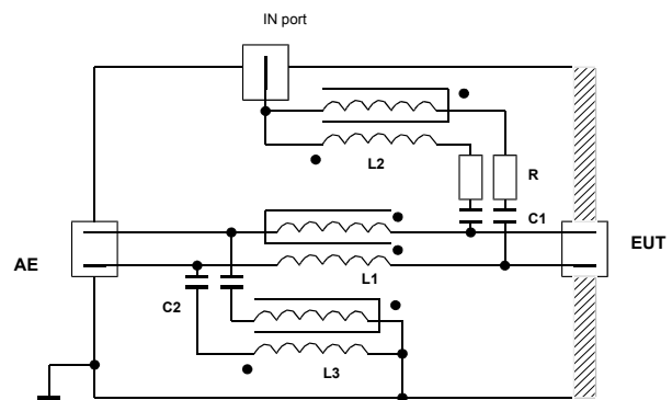
Circuit diagram CDN T2
