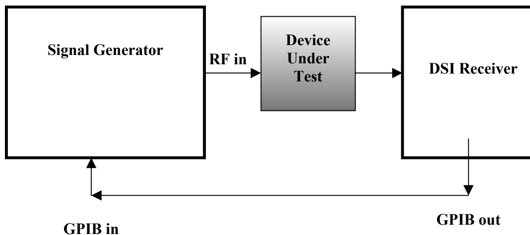
Figure 3. Swept frequency tracking with a DSI Receiver
